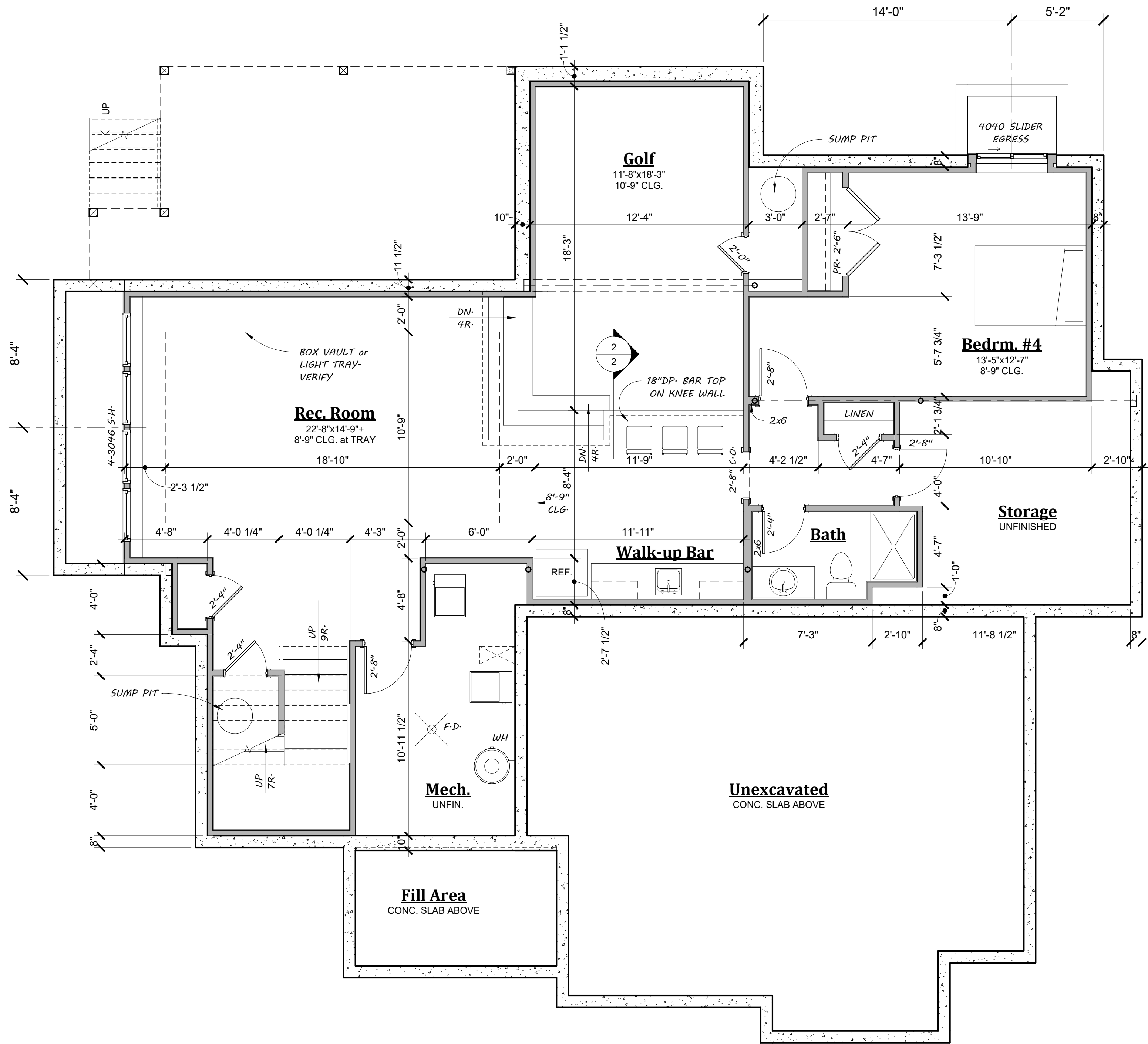
1 Basement Finish Plan 1/4" = 1'-0"
